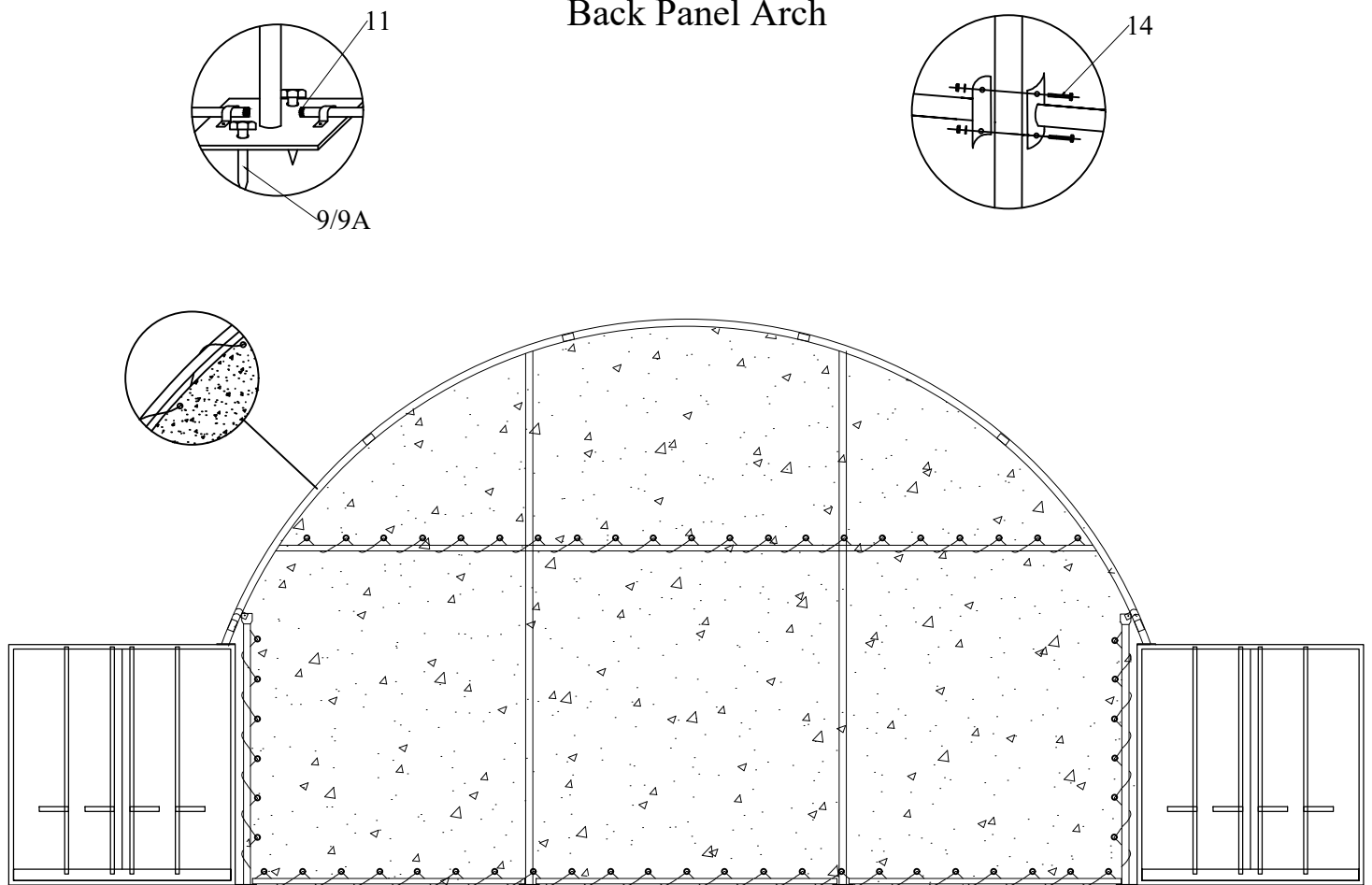
Installation of Back Panel Cover
